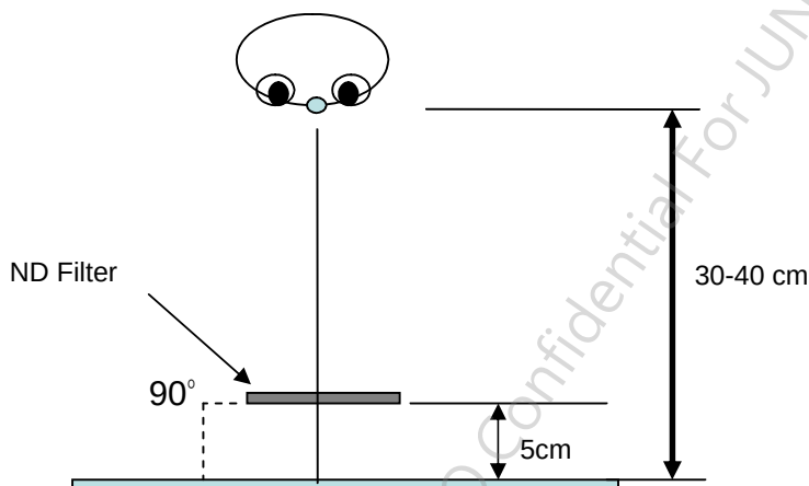
Note 7) Defect criteria diagram
